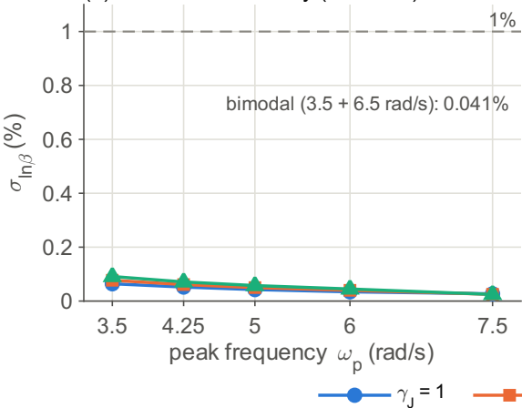
(a) Stiffness uncertainty ( L = 2048 )
