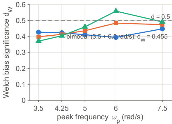
(b) Welch bias ( L = 2048 )
